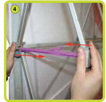
4 Push fit together each pair of locking arms. Repeat for all the remaining arms.
